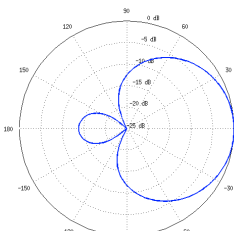
H-Pol Elevation
