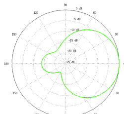
H-Pol Azimuth
