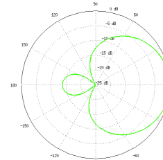
V-Pol Azimuth
