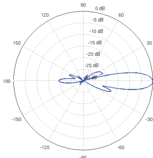
Vertical Elevation
