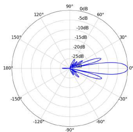
Horizontal Elevation
