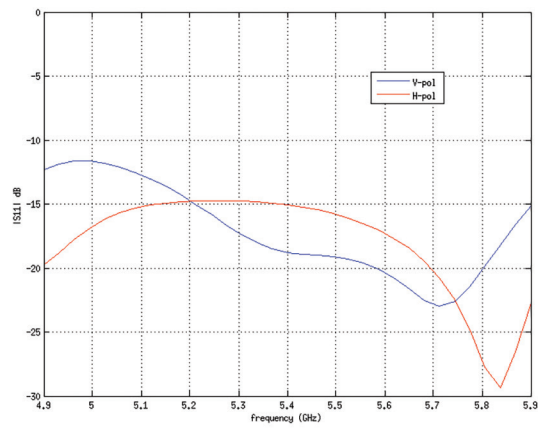
Return Loss
