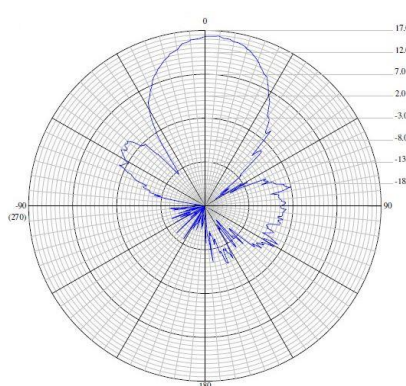
EZ-Bridge®-LT+HD Antenna Patterns
