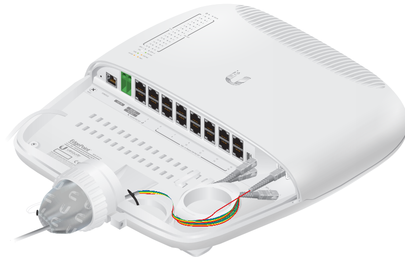
EP-S16 Strain Relief for Fiber Optic Strands
