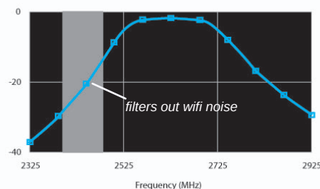
Receiver Frequency Response
