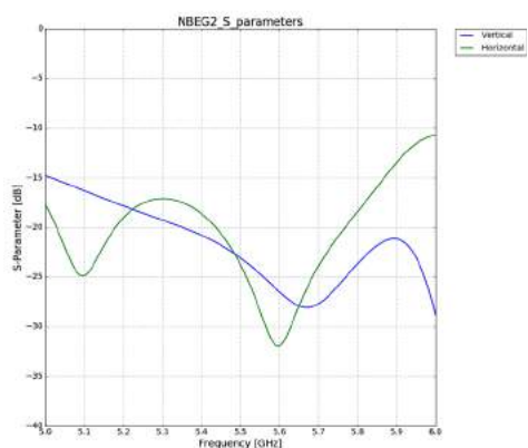
Return Loss
