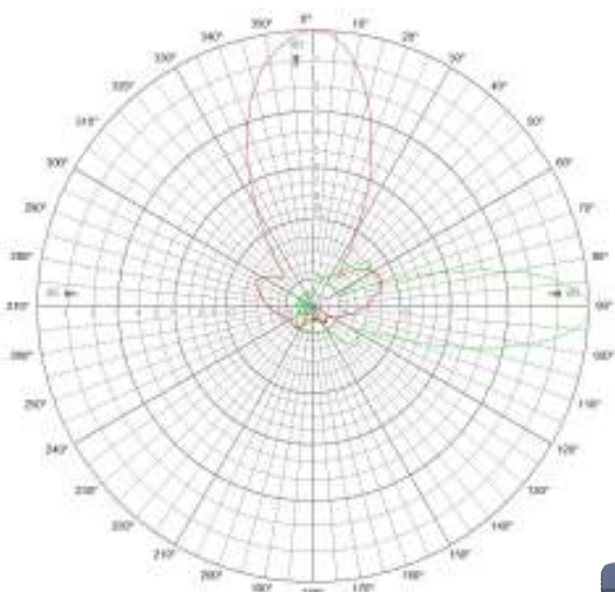
EZ-Go-2 14dBi Antenna Pattern
