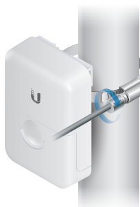
1. Attach the ETH-SP-G2 to a grounded pole.
